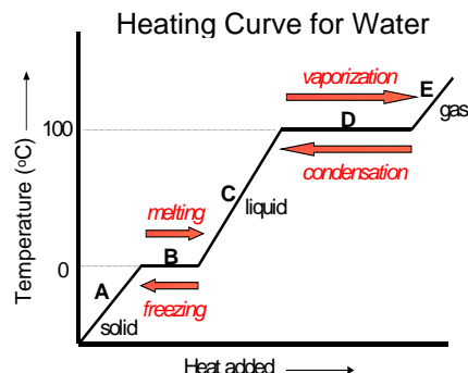
Energy Changes Accompanying Phase Changes
